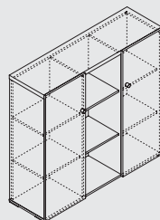
MIT20 1363 | 418 | 1280 53 5/8" | 16 1/2" | 50 3/8"
